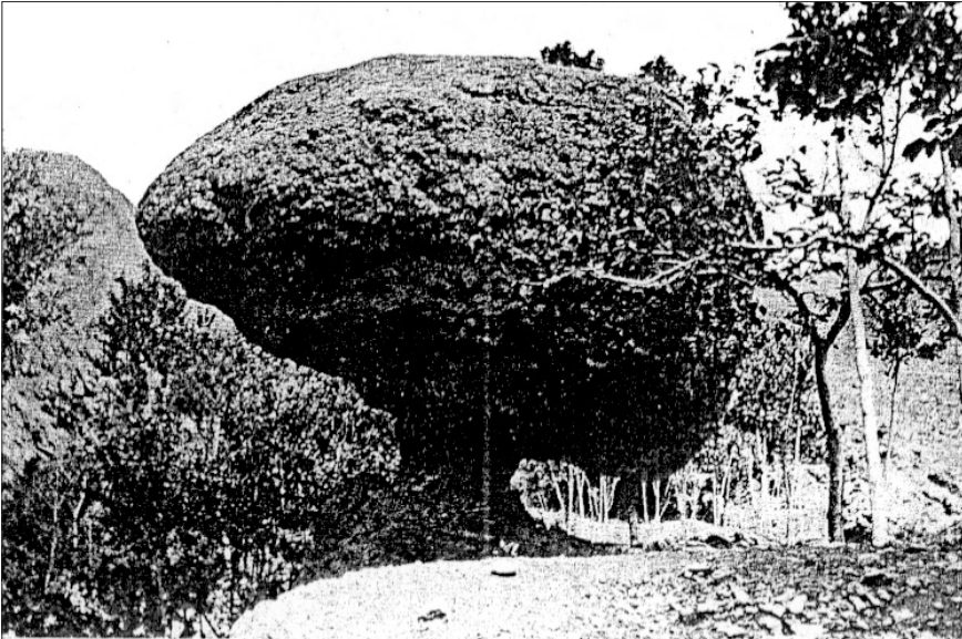
The Mushroom Rock at Villenjach, near Tajreesh.
